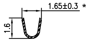
B-B SECTION
