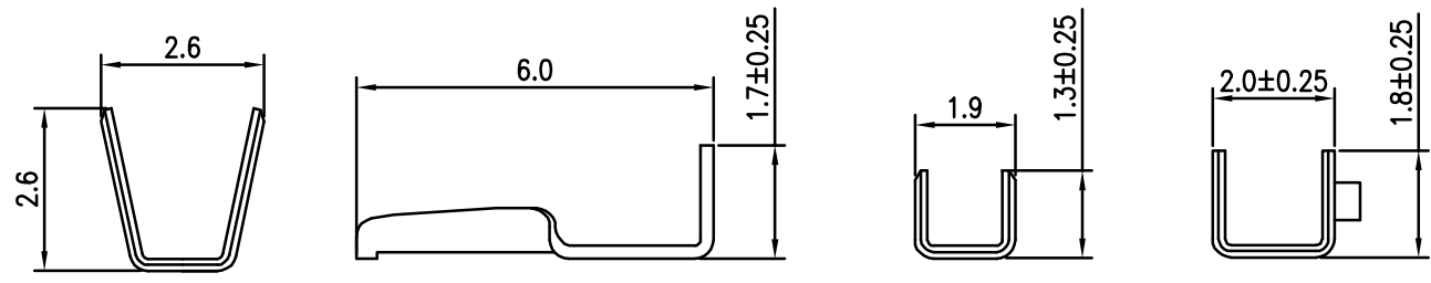
SECTION A-A SECTION B-B SECTION C-C SECTION D-D
