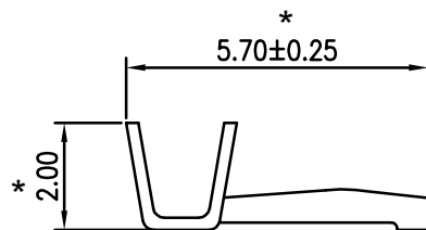
B-B SECTION
